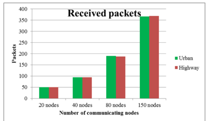
Fig. 9. Received packets for Urban and Highway scenarios with algorithm.
