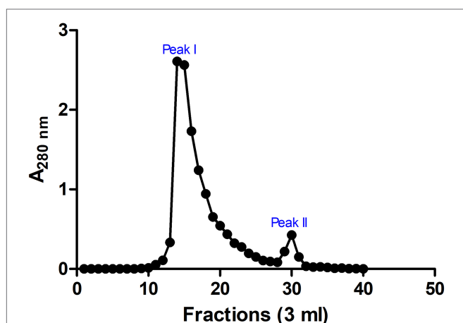
FIGURE 3 | Chromatogram for fractions of gel filtration chromatography. Sephadex G-25 chromatographic resin was used and two prominent peaks (peaks I and II) were observed. Absorbance was measured at 280 nm. The image was rendered in GraphPad 5.0 statistical package.
