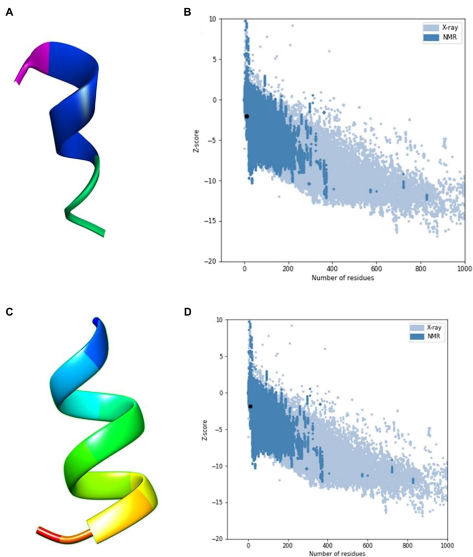
FIGURE 5 | AWSEM and PEP-FOLD predicted peptide 3D structures of ACAP-I together with respective ProSA validation plots. (A) AWSEM-modeled ACAP-I predicted 3D structure, (B) AWSEM modeled ACAP-I ProSA z-score, (C) PEP-FOLD-modeled ACAP-I 3D structure, (D) PEP-FOLD-modeled ACAP-I ProSA z-score. AWSEM modeled ACAP-I and PEP-FOLD-modeled ACAP-I peptide had z-scores of -1.99 and -1.85 , respectively, and were within the normal z-score of experimentally validated proteins.
