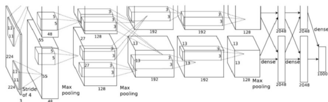
FIGURE 4. The AlexNet Architecture.
