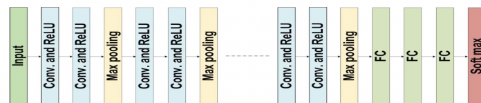
FIGURE 5. The VGG Architecture.
