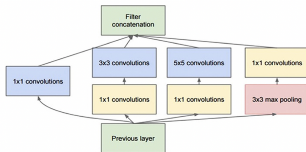
FIGURE 6. The inception module in GoogLeNet [106].
