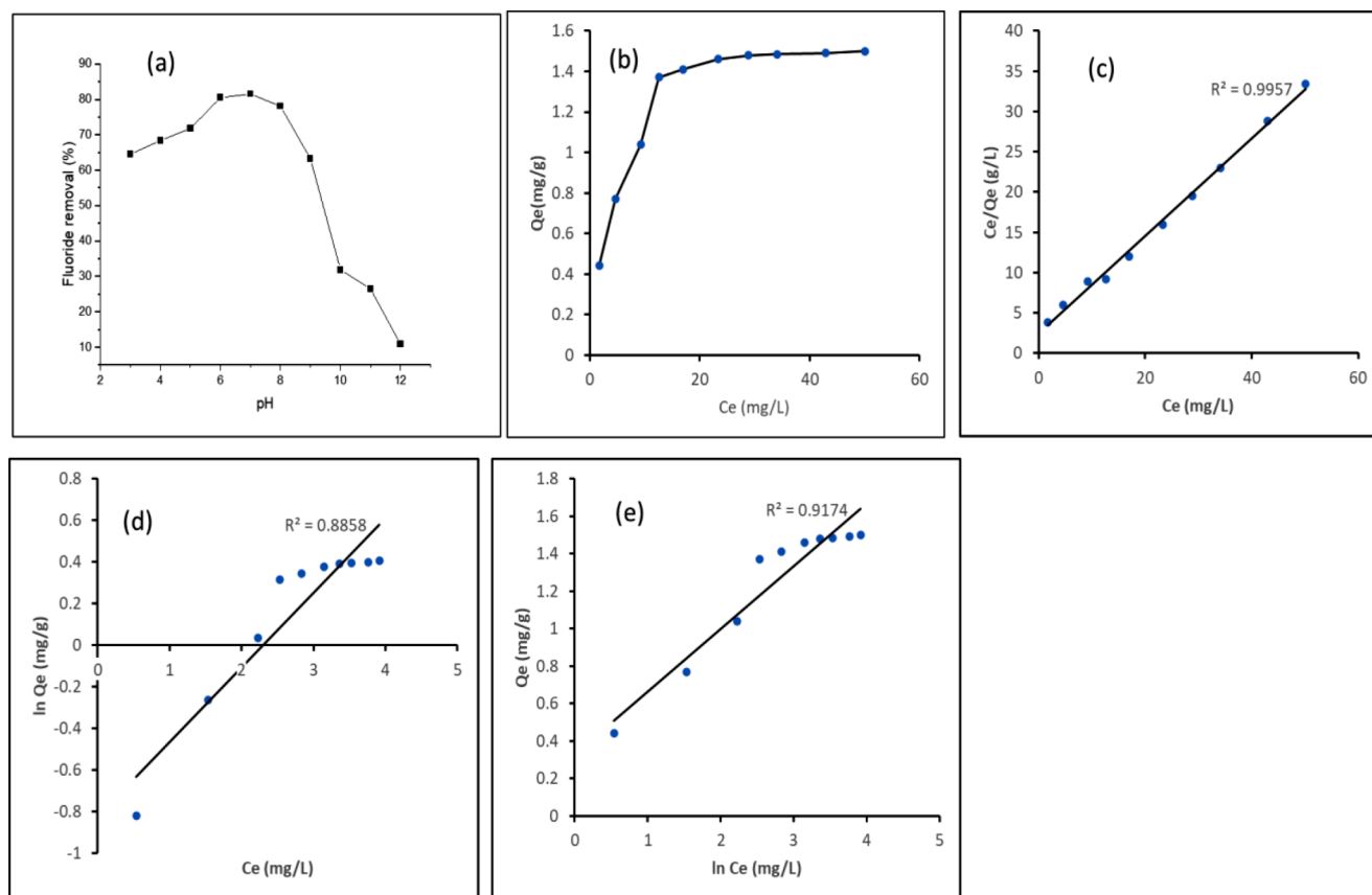
Fig. 4. Sorption equilibrium study of fluoride onto \alpha\text{-Fe}_2\text{O}_3 biocomposite: (a) effect of pH on fluoride removal (b) variation of sorption with respect to change of the initial concentration of fluoride (c) Langmuir isotherm (d) Freundlich isotherm (e) Temkin isotherm.
