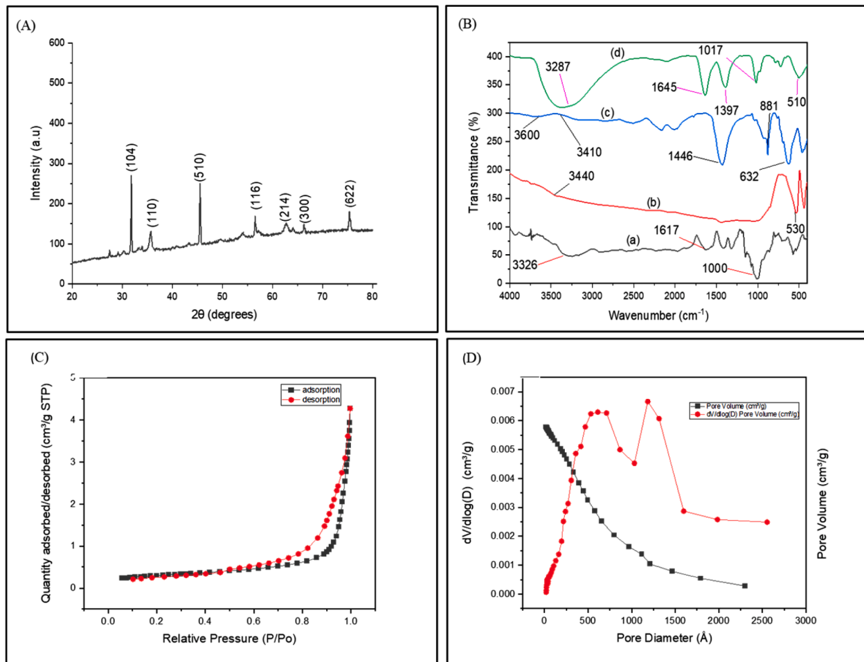
Fig 3. (A) XRD spectra of \alpha\text{-Fe}_2\text{O}_3 biocomposite (B) FTIR spectra of (a) pristine cassava starch (CS) (b) \alpha\text{-Fe}_2\text{O}_3 -prepared using 0 CS (c) \alpha\text{-Fe}_2\text{O}_3 biocomposite (d) \alpha\text{-Fe}_2\text{O}_3 composite-F (C) BET plot of nitrogen adsorption-desorption for \alpha\text{-Fe}_2\text{O}_3 biocomposite (D) pore size distribution of \alpha\text{-Fe}_2\text{O}_3 biocomposite obtained by BJH method.
